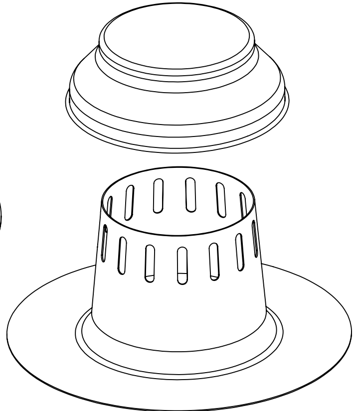
EXPLODED VIEW
