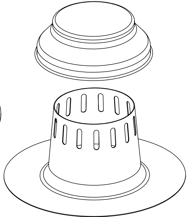
EXPLODED VIEW
